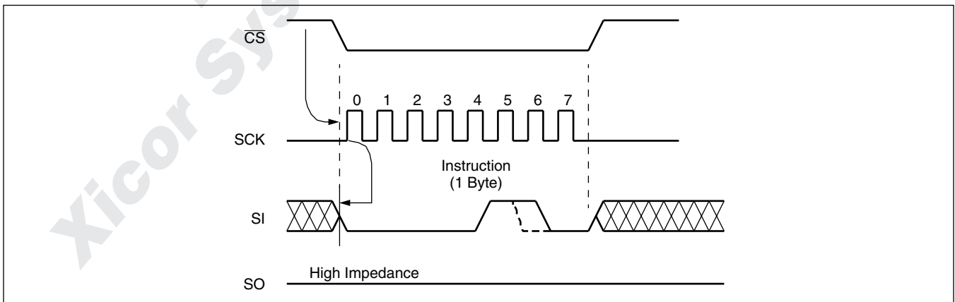
Figure 3. WREN/WRDI Sequence
