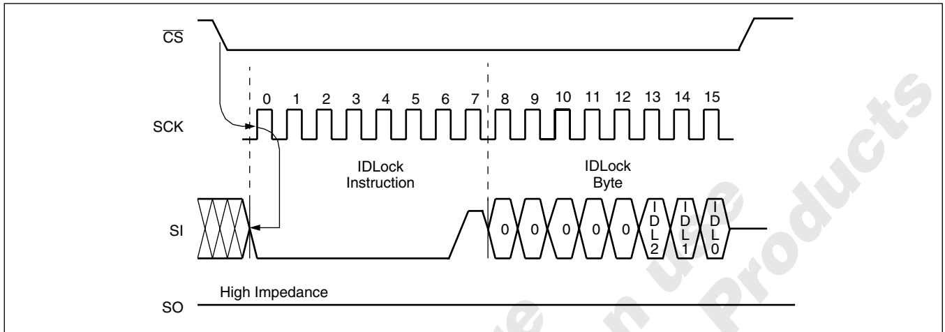
Figure 6. IDLock Operation Sequence
